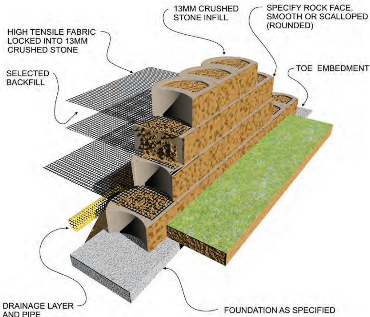
COMPOSITE STRUCTURE
